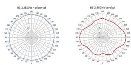
FAP-233G Radio3 antenna plots
